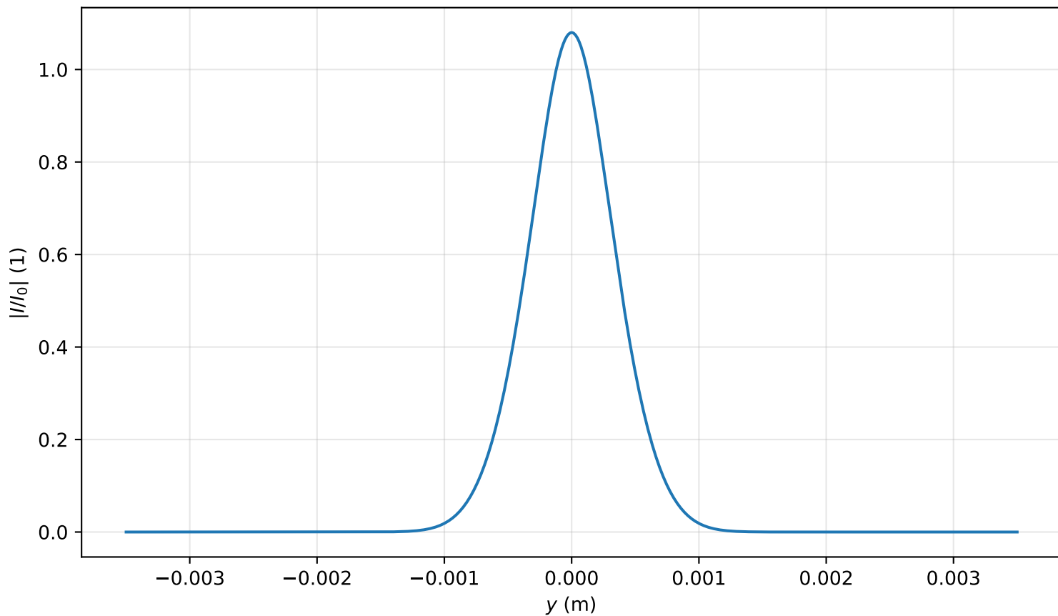
Intensity profile I(x=0, y, z=0.398)/I_0 , P_{in}=0.8P_{cr} , artificial time
